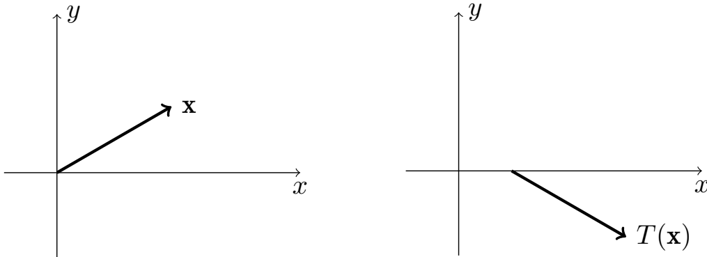
Figure 12.12 Glide reflections
