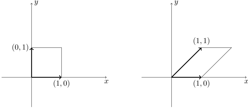
Figure 12.4 SL_2(\mathbb{R}) acting on the unit square
